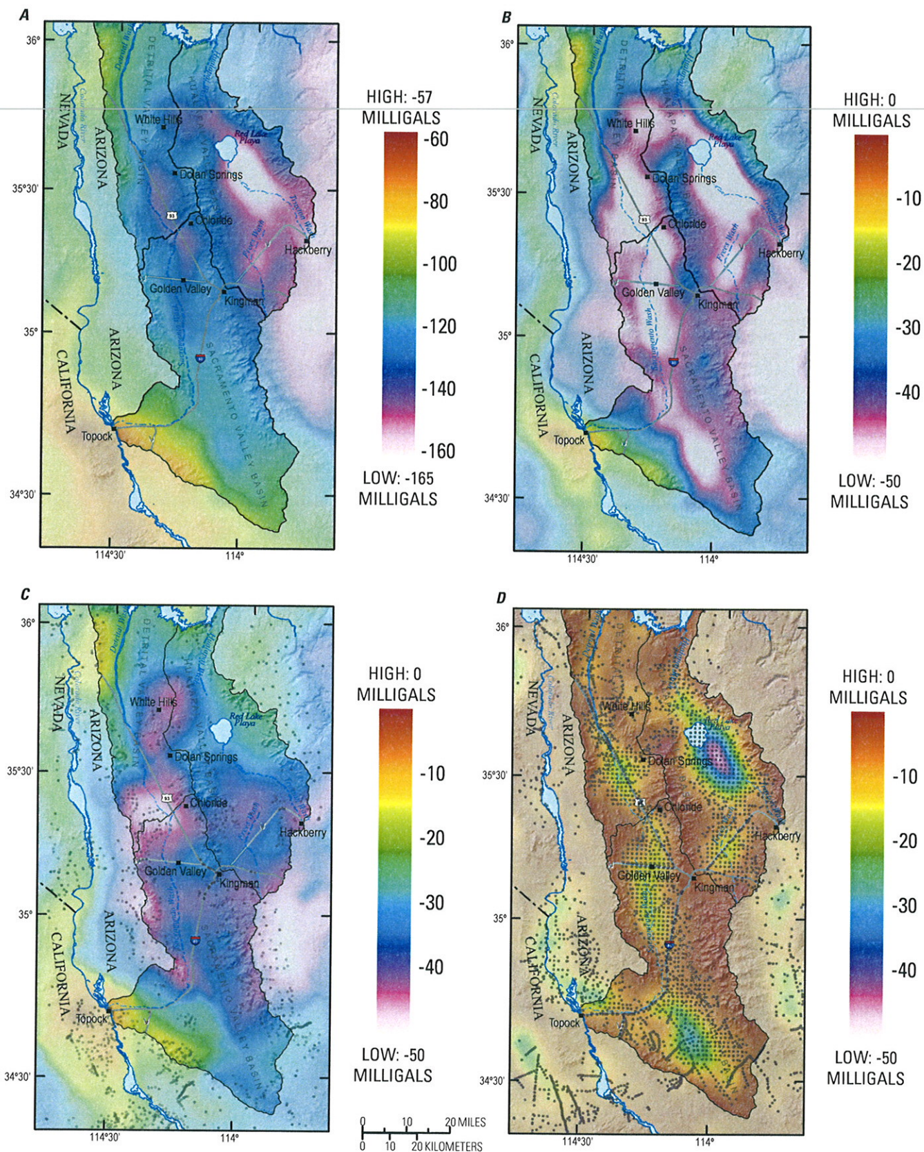
Figure 8. Basin gravity anomaly in Mohave County, northwest Arizona. A , Complete Bouguer anomaly. B , Isostatic residual anomaly. C , Bedrock residual anomaly. D , Basin residual anomaly. Gray circles indicate position of gravity measurements. All grids are upward-continued to 2,550 m elevation. Color scale for figures B through D is identical.
