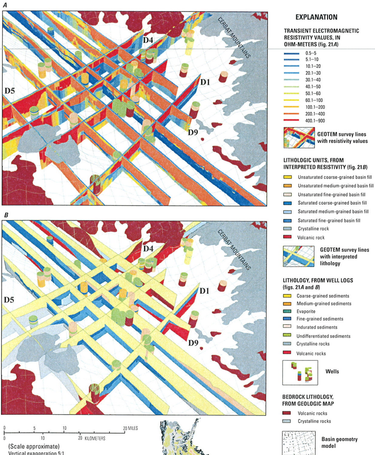
Figure 21. Mohave County, northwest Arizona, showing perspective view to the northeast of uninterpreted (A) and interpreted resistivity (B) from GEOTEM profiles in the southern Detrital subbasin in Detrital Valley basin. Interpretation of resistivity may differ along profiles that are perpendicular to one another, suggesting that the basin fill may be interlayered and (or) a factor of the resistivity modeling where some surface interference may have occurred or overlying lithology attenuated signal. Profiles are numbered in the same order as in figure 11.
