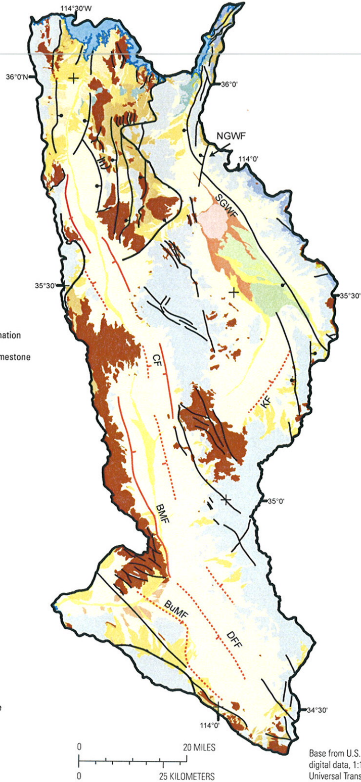
Figure 3. Mohave County, northwest Arizona, showing surface geology and structure in Hualapai Valley, Detrital Valley, and Sacramento Valley basins. Mapped faults are shown in black; black hachured lines are low-angle detachment faults. Faults inferred from basin geometry model gravity model and transient electromagnetic data shown in red. Dashed red lines denote higher degree of uncertainty (BGF, Blind Goddess Fault; BMF, Black Mountain Fault; BuMF, Buck Mountain Fault; CF, Chloride Fault; DDF, Dutch Flat Fault; KF, Kingman Fault; NGWF, northern section of the Grand Wash Fault; SGWF, southern section of the Grand Wash Fault).
